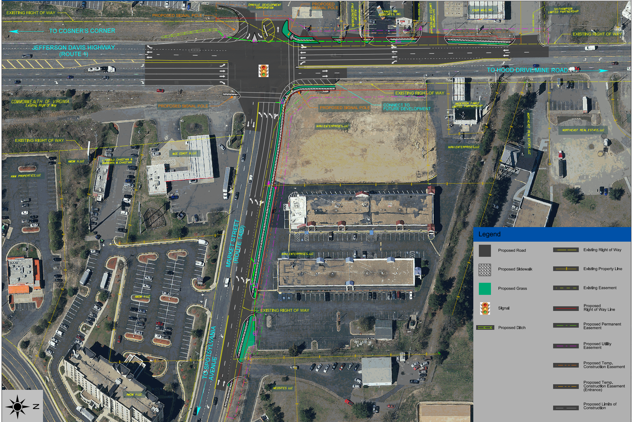
Route 1 and Market Street Turn Lanes Spotsylvania County, Virginia
