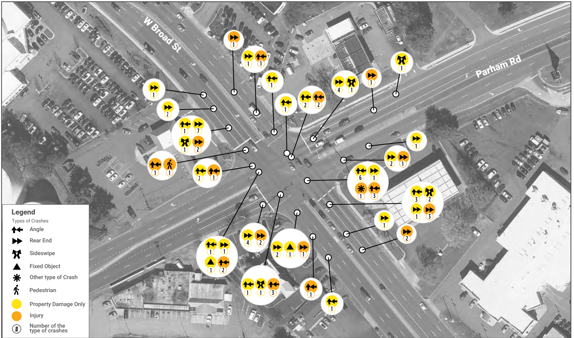
W. Broad Street and Parham Road Crash Diagram (2016-2020)
