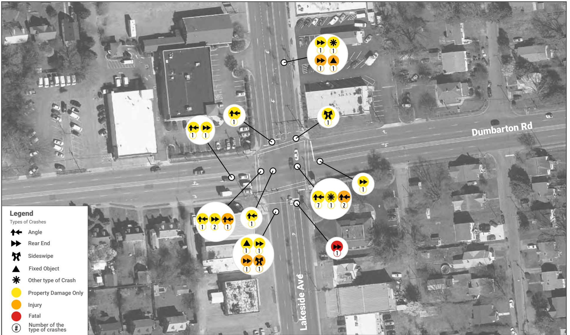
Lakeside Avenue and Dumbarton Road Crash Diagram (2016-2020)
