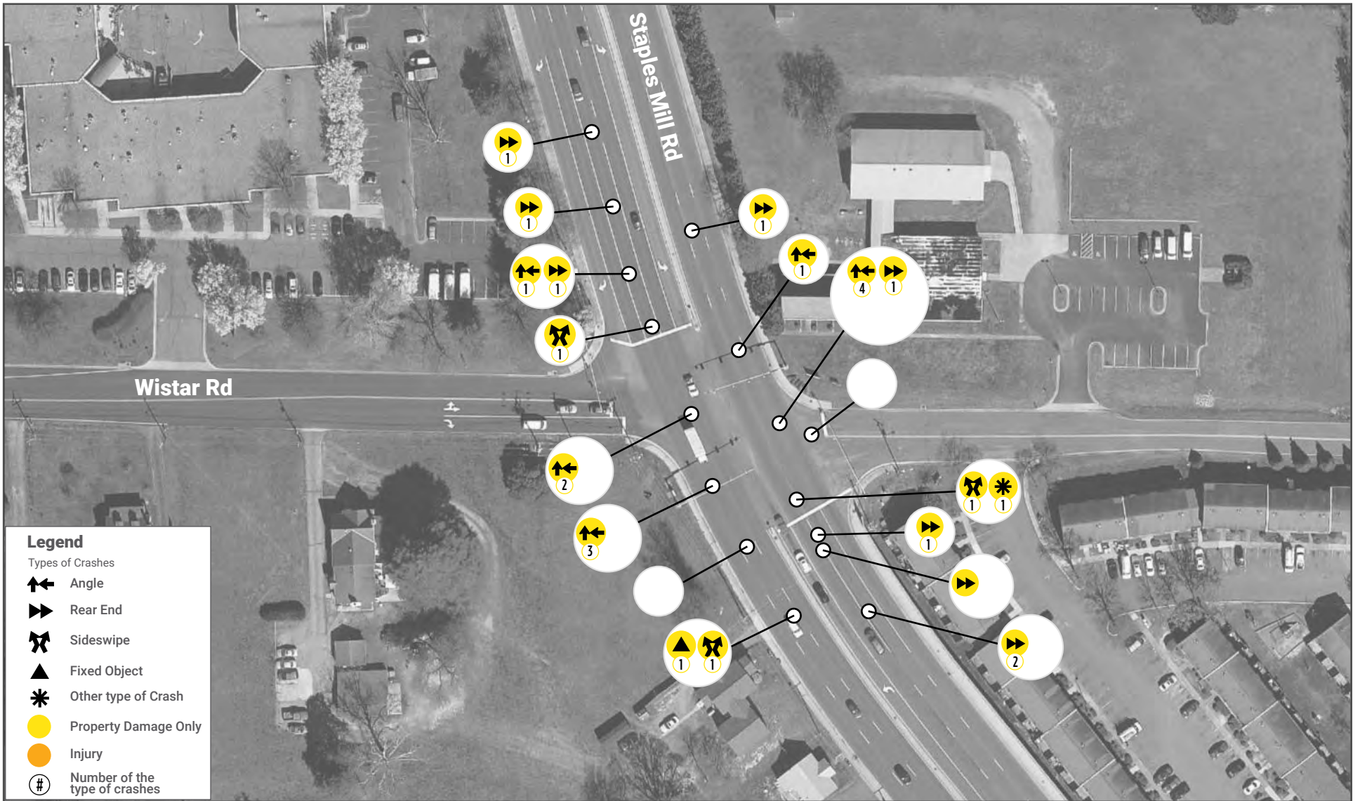
Staples Mill Road and Wistar Road Crash Diagram (2016-2020)
