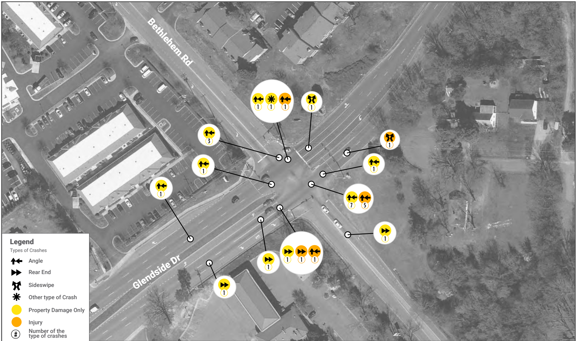
Glenside Drive and Bethlehem Road Crash Diagram (2016-2020)
