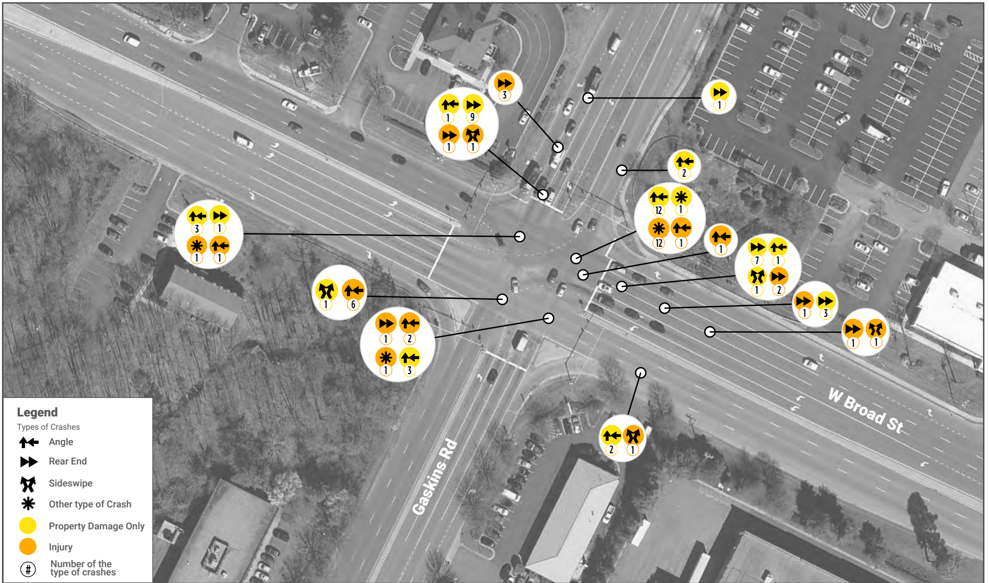
W. Broad Street and Gaskins Road Crash Diagram (2016-2020)
