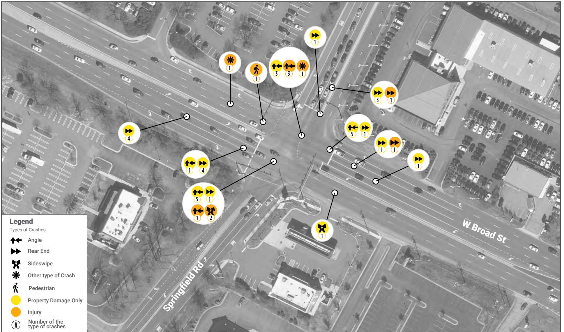
W. Broad Street and Pemberton Road/Springfield Road Crash Diagram (2016-2020)
