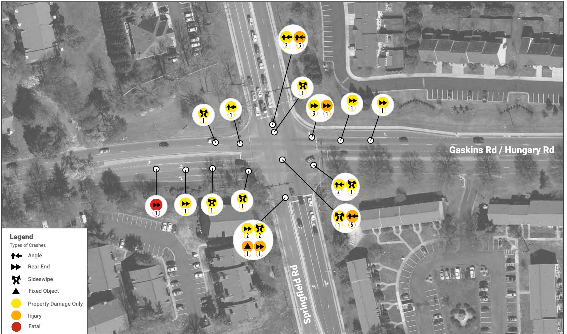
Springfield Road and Gaskins Road/Hungary Road Crash Diagram (2016-2020)
