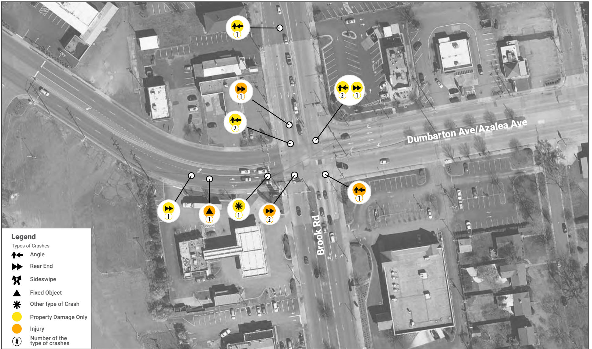
Brook Road and Dumbarton Avenue/Azalea Avenue Crash Diagram (2016-2020)
