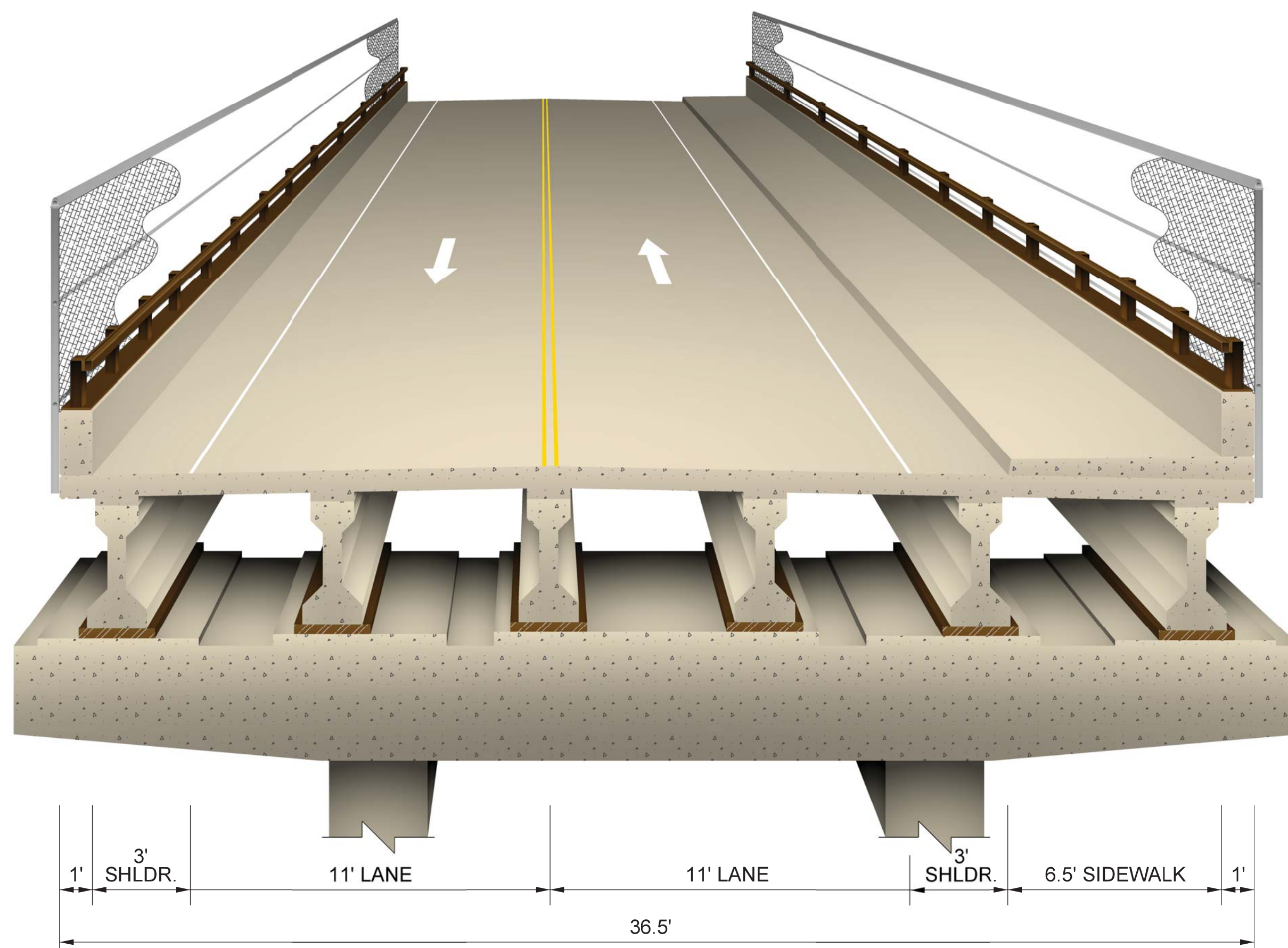
Typical Bridge Section (Looking North)
